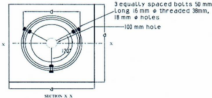
DETAILS OF MS BASE PLATE (Separately packed)
