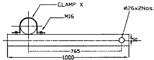
TOP CROSS ARM ASSEMBLY (SMC 100x50 (1 no))
