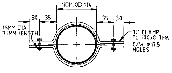
4 STAY CLAMP
