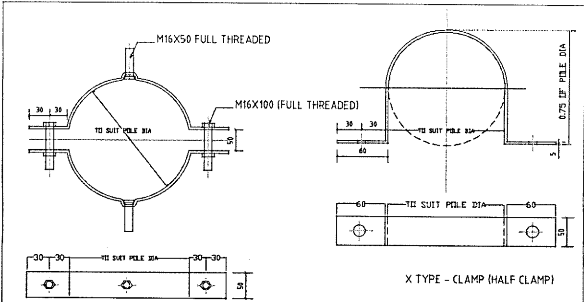
Y TYPE - CLAMP (FULL CLAMP)
