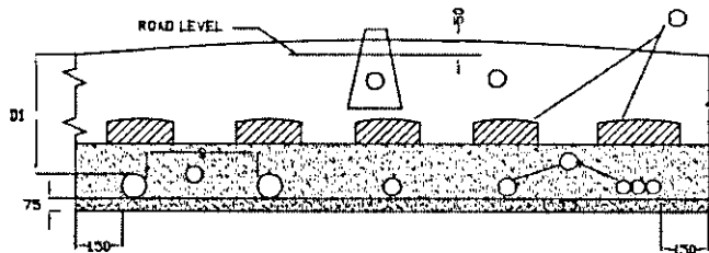
DIRECTLY BURIED CABLES IN SINGLE LAYER
