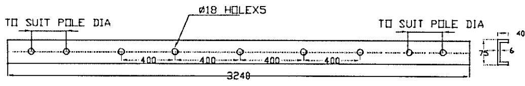
EQUIPMENT CROSSARM CHANNEL (ISMC 75x40x6) - 3 NOS
