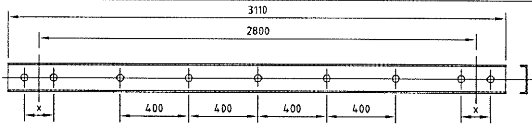
EQUIPMENT SUPPORTS, CH 75x40 (3NOS)
