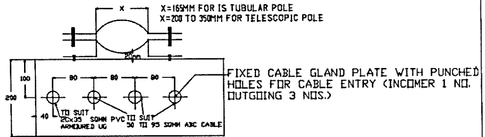
BOTTOM VIEW
