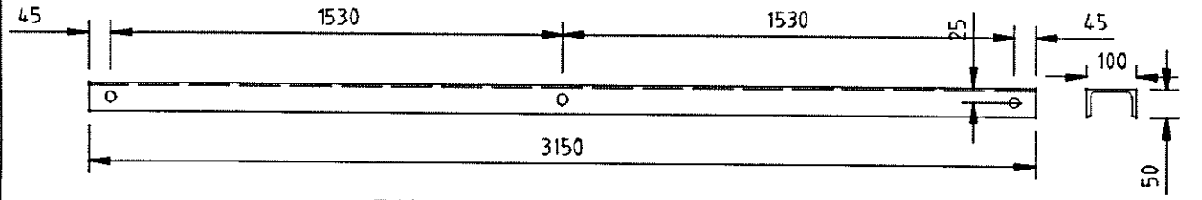
TOP VIEW OF CROSSARM - CHL ISMC 100x50 (2 NOS)
