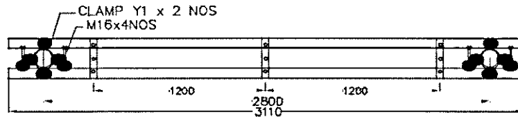
CROSSARM ASSEMBLY
