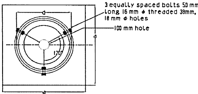
DETAILS OF MS BASE PLATE (Separately packed)
