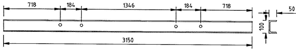
FRONT VIEW OF CROSSARM - CHL ISMC 100x50 (2 NOS)
