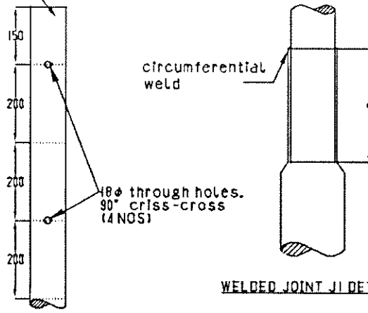
POLE TOP DETAILS
