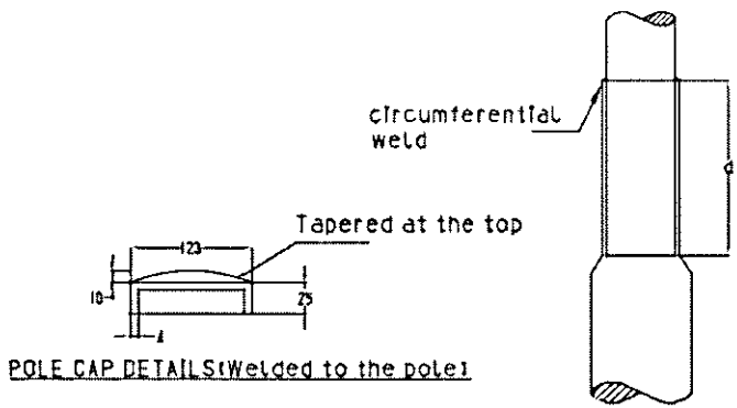
WELDED JOINT J1 DETAILS
