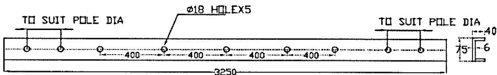
EQUIPMENT CROSSARM CHANNEL (ISMC 75x40) - 3 NOS
