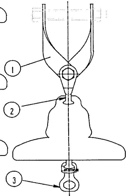
11 kV SINGLE TENSION STRING
