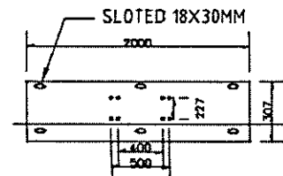
PLATFORM REST PLATE (2000X307X5)
