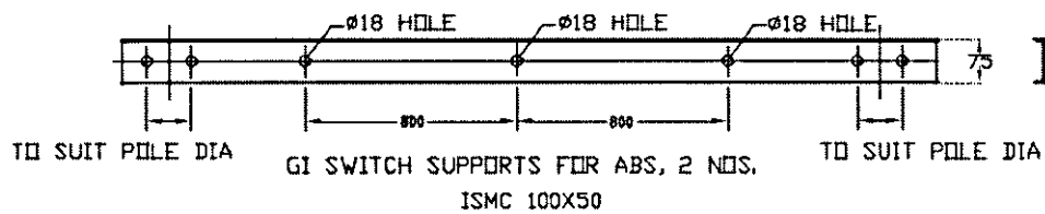
CROSSARM CHANNEL (ISM 100x50) - PLAN
