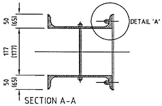
TRANSFORMER BELTING L HOOK 75x75MM (ANGLE 50x65MM)
