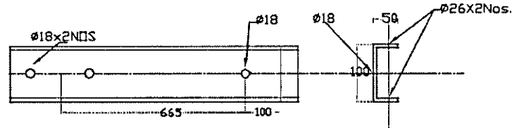
TOP CROSS ARM CHANNEL (SMC 100x50x1000) - 1 NO
