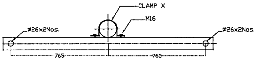
LOWER CROSS ARM ASSEMBLY (SMC 100x50 (1 no.))
