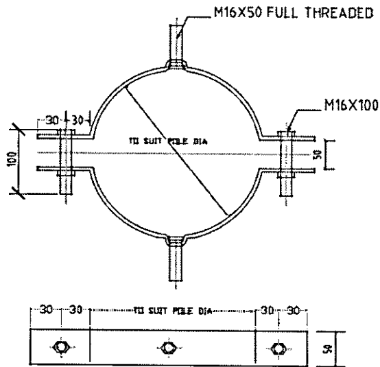
STAY CLAMP
