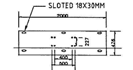
PLATFORM REST PLATE (2000X307X5)
