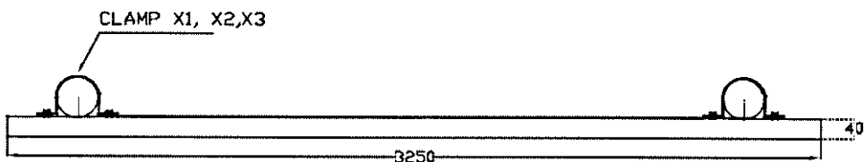
CROSSARM CHANNEL (ISMC 100x50) - PLAN
