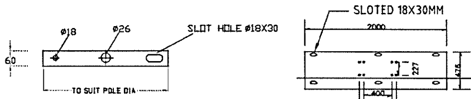
MS TENSION STRAP (60x6) - 6 NOS
