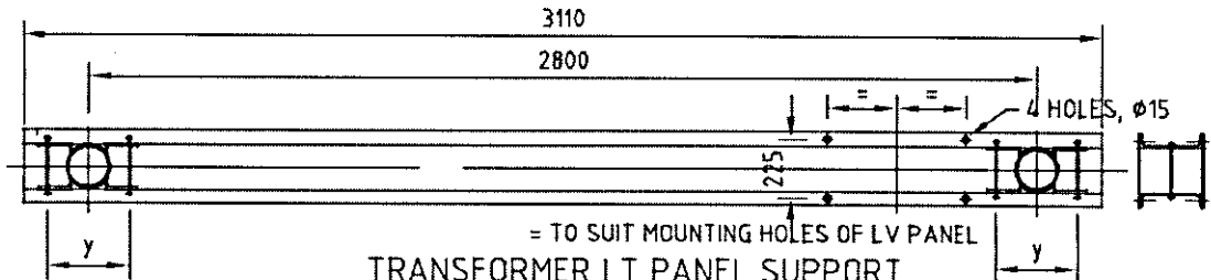
EQUIPMENT SUPPORTS, CH 75x40 (3NOS)
