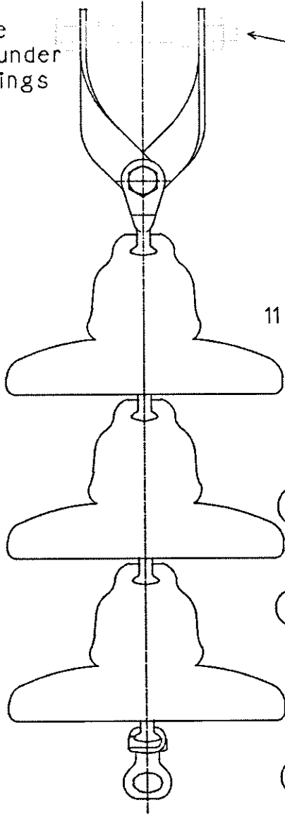
33 kV SINGLE TENSION STRING
