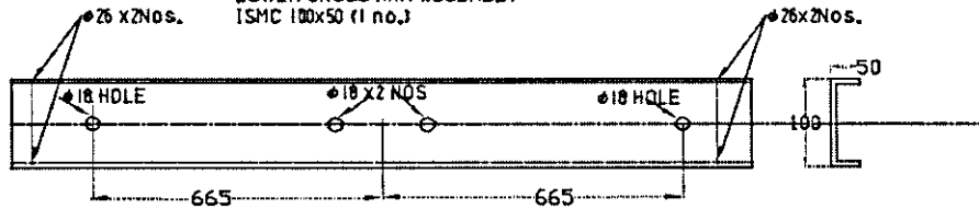
LOWER CROSS ARM CHANNEL (SMC 100x50x1650) - 1 NO
