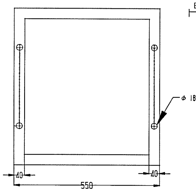
FOUNDATION PLAN
