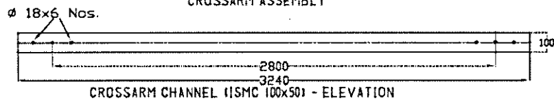
CROSSARM CHANNEL (ISM 100x50) - ELEVATION
