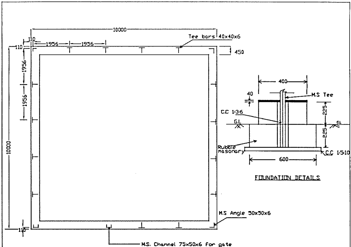
PLAN TRANSFORMER YARD FENCING 10M x 10M (N.T.S)
