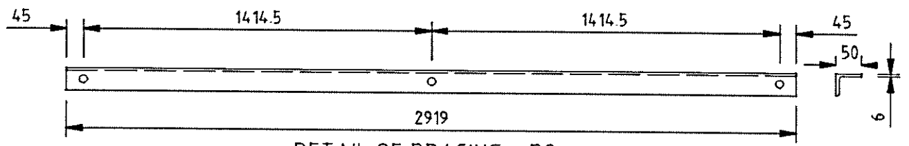
DETAIL OF BRACING - B2 ISA 50x50x6 (2 NOS)
