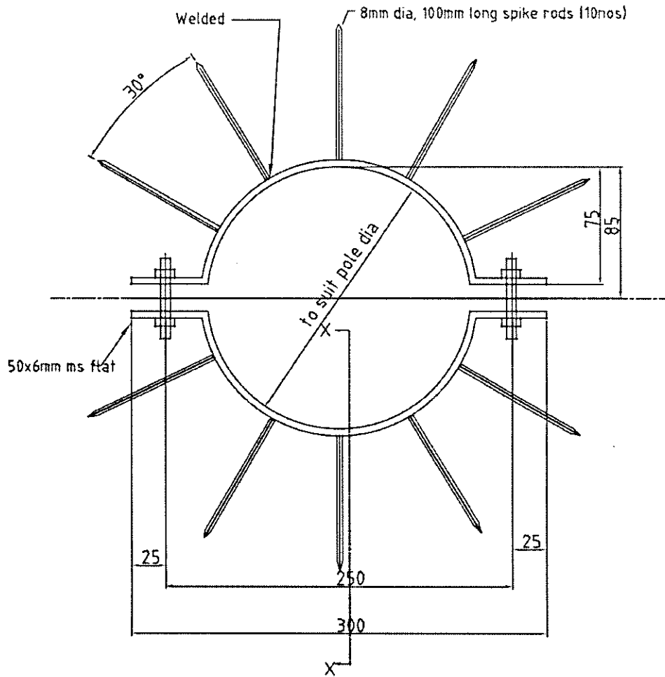
section X-X
