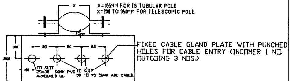
BOTTOM VIEW
