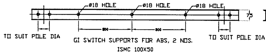
CROSSARM CHANNEL (ISMC 100x50) - PLAN
