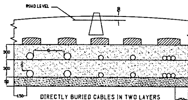
DIRECTLY BURIED CABLES IN TWO LAYERS
