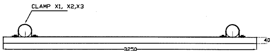
CROSSARM CHANNEL (ISM 100x50) - PLAN
