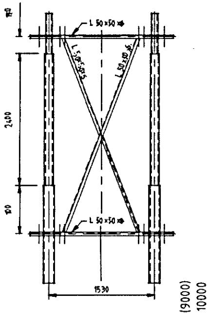
BRACING ASSEMBLY DETAILS
