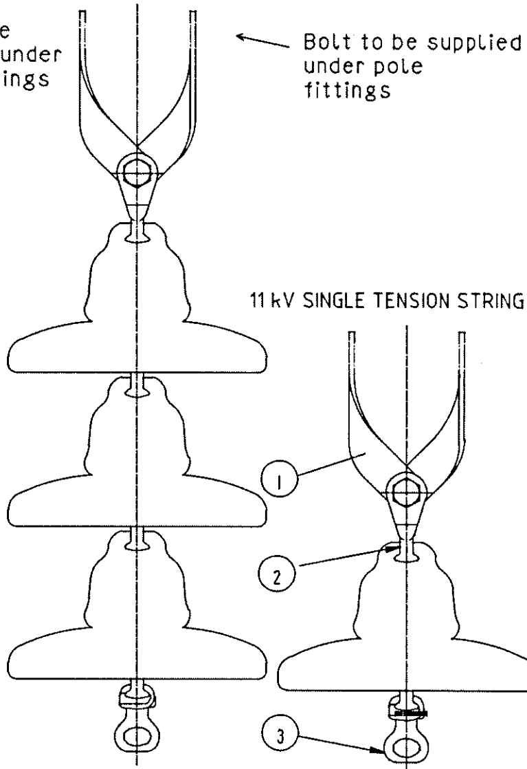
33 kV SINGLE TENSION STRING
