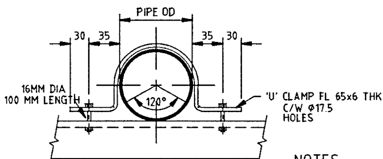
3 FULL CLAMP
