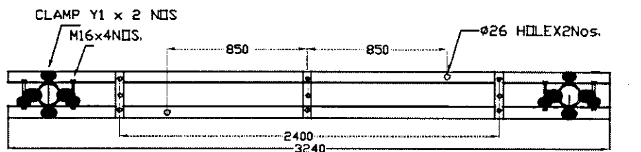
TOP CROSSARM ASSEMBLY
