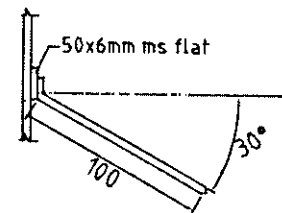
section X-X
