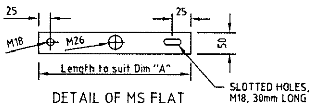
DETAIL OF MS FLAT FL 50x6 (6 NOS) GI 16MM DIA NUTS AND BOLTS (6NOS)
