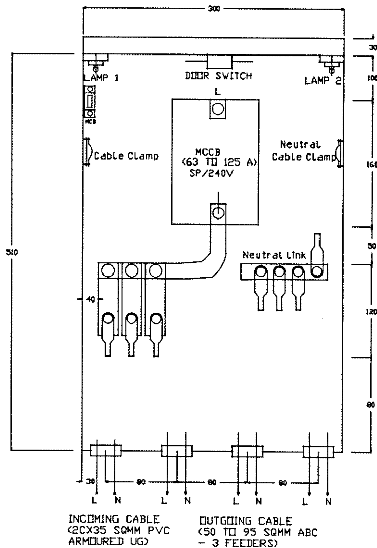
INTERNAL WIRING DIAGRAM OF DISTRIBUTION PILLAR
