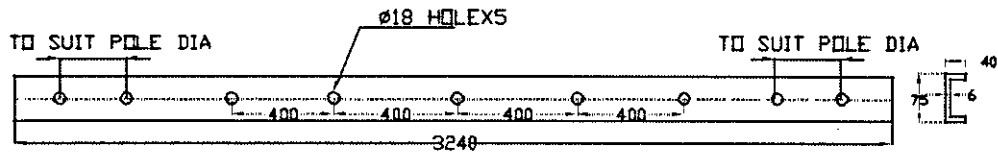
EQUIPMENT CROSSARM CHANNEL (ISMC 75x40x6) - 3 NOS
