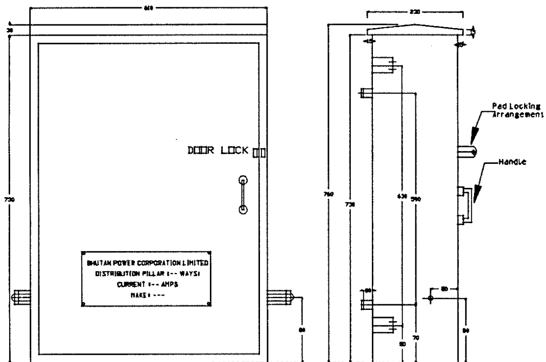
SIDE VIEW
