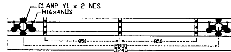
CROSSARM ASSEMBLY
