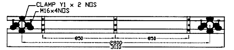
CROSSARM ASSEMBLY
