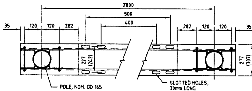
ARCB & PT PLATFORM (2Nos.) ISMC 125x65
