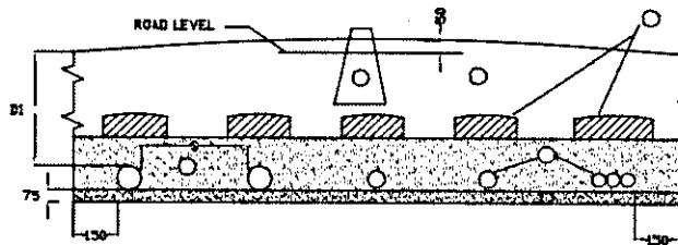
DIRECTLY BURIED CABLES IN SINGLE LAYER
