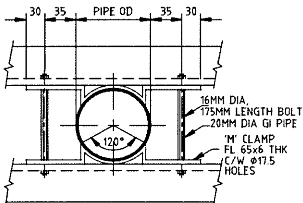
2 'M' CLAMP
