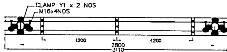
CROSSARM ASSEMBLY
