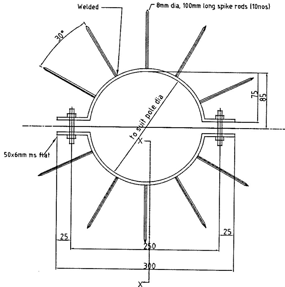
section X-X
