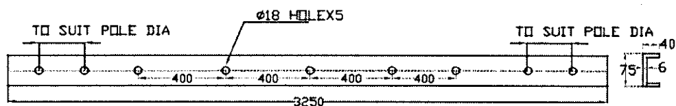
EQUIPMENT CROSSARM CHANNEL (ISM 75x40) - 3 NOS
