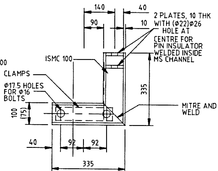
TOP HAMPER FOR INSULATOR PIN DETAIL
