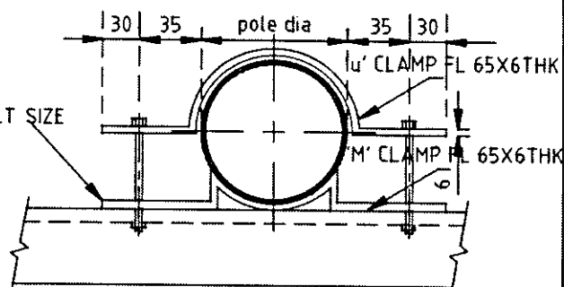
CLAMP DETAILS (U+M) (2 sets)
