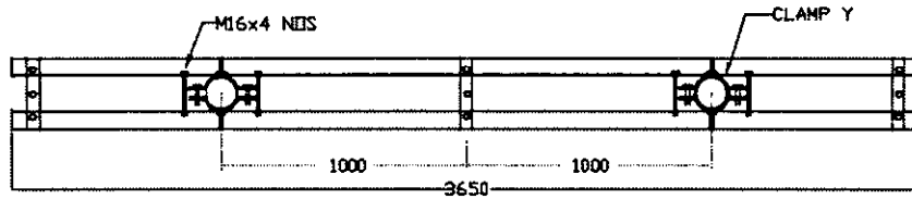
CROSS ARM ASSEMBLY PLAN
