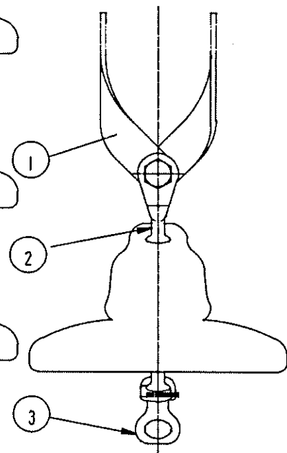
11 kV SINGLE TENSION STRING
