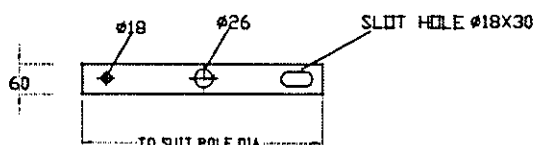
MS TENSION STRAP (60x6) - 5 NOS
