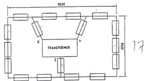
RECTANGULAR ARRANGEMENT
