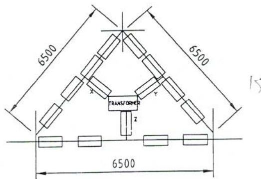
TRIANGULAR ARRANGEMENT
