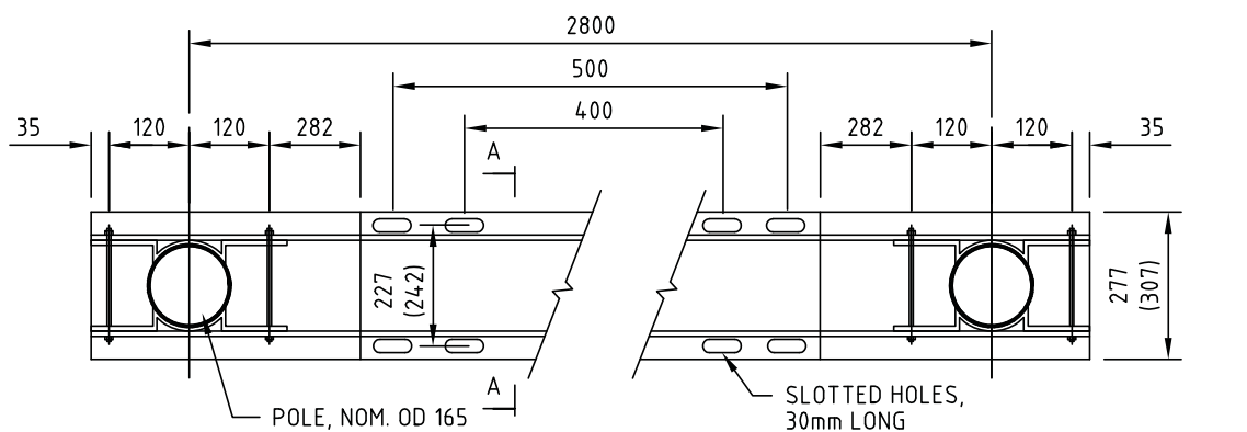
TRANSFORMER PLATFORM (2Nos.) ISM 125x65
