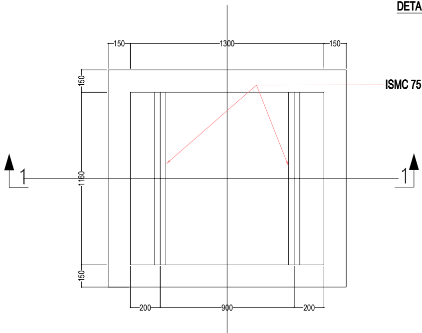
FOUNDATION PLAN
