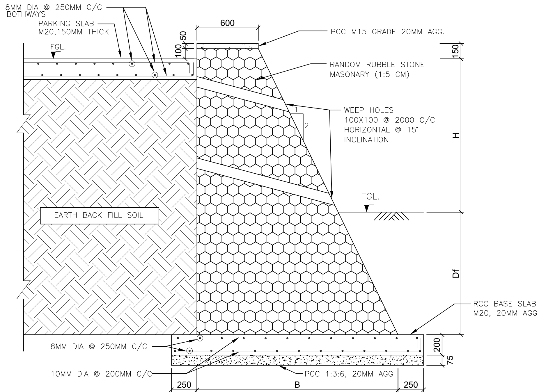
RANDOM RUBBLE MASONRY WALL FOR 'H' HEIGHT
