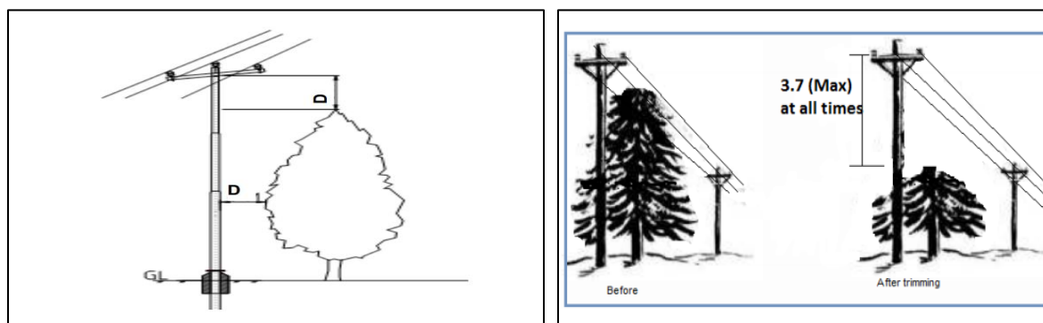
Fig. 2 Top Trimming
