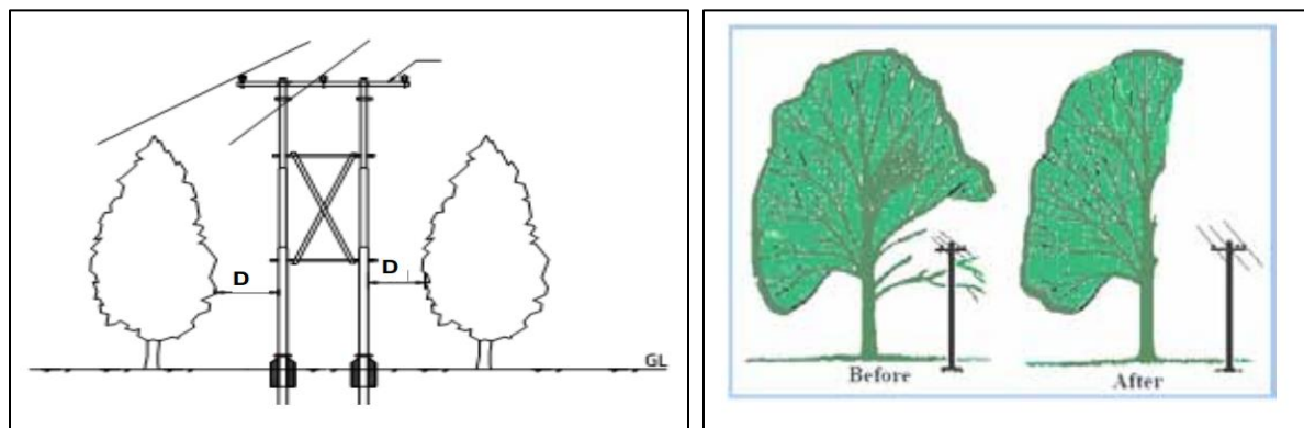
Fig. 1 Side Trimming
