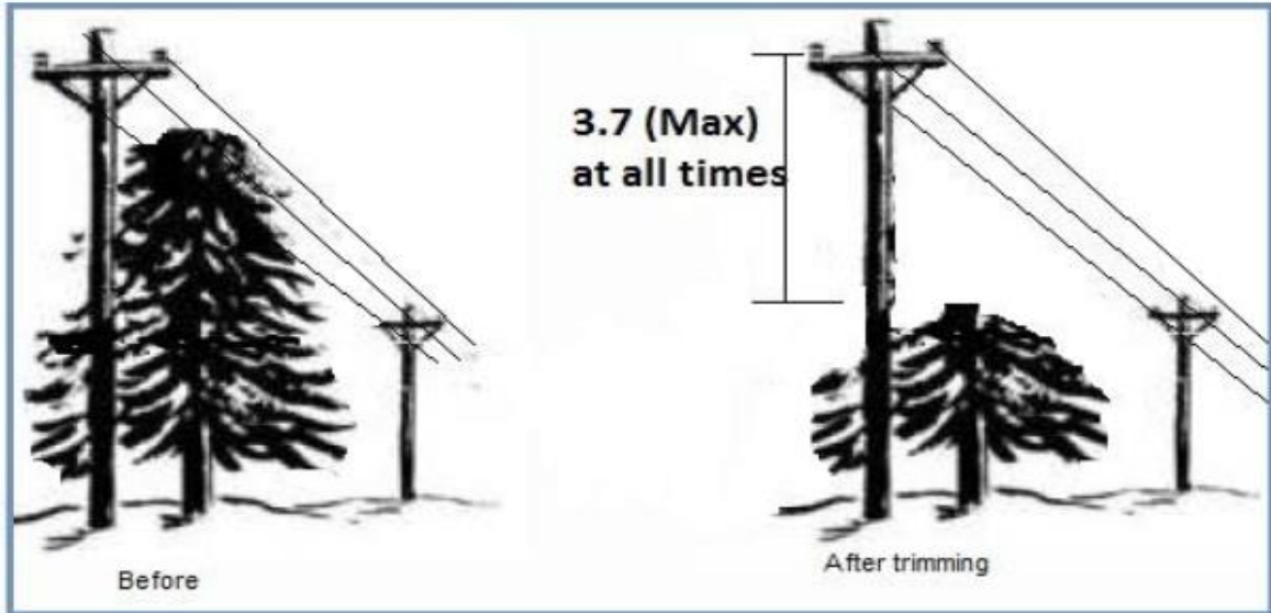
Fig-1: Top Trimming for MV Lines
