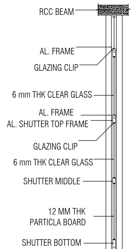
SECTION XX
