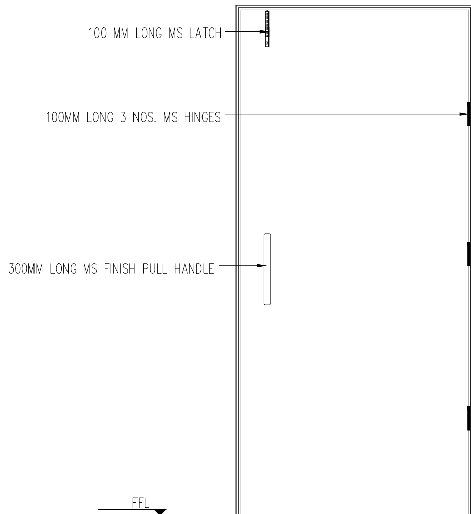
ELEVATION INSIDE
