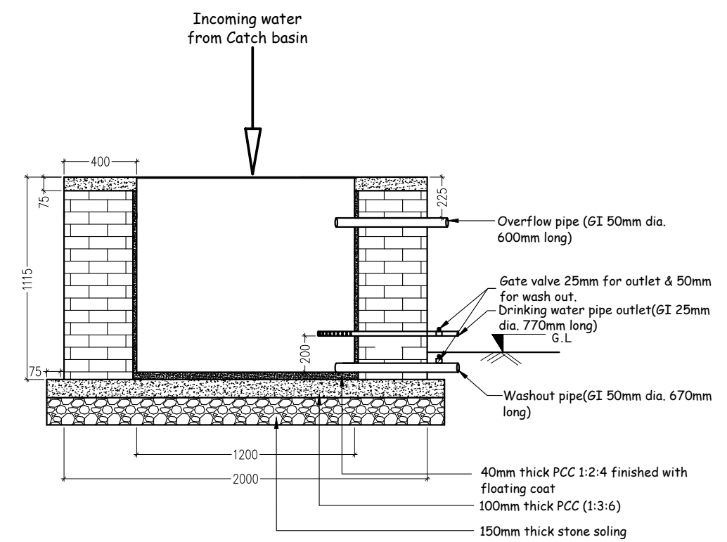
TYPICAL SECTION OF INTAKE WATER TANK
