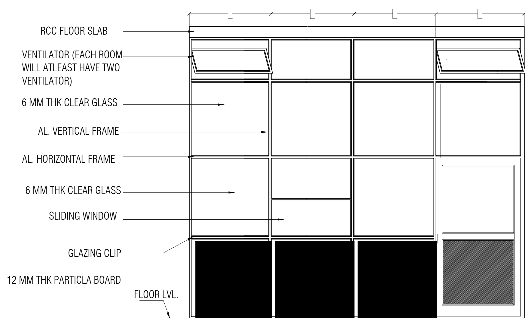
TYPICAL DETAIL FOR INTERIOR ALUMINUM-GLAZING PARTITION
