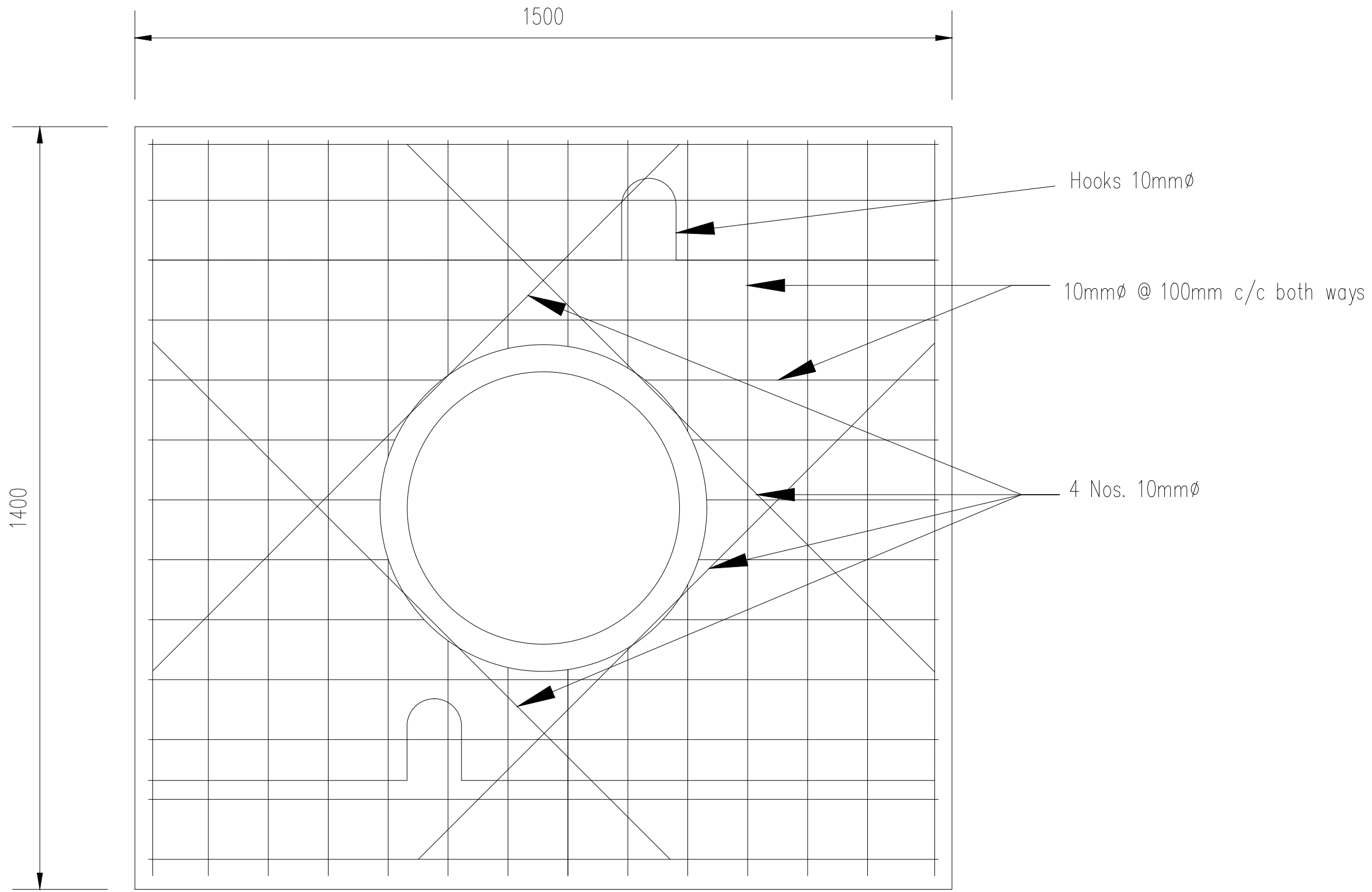
TOP SLAB, GRADE 20 CONCRETE – PLAN
