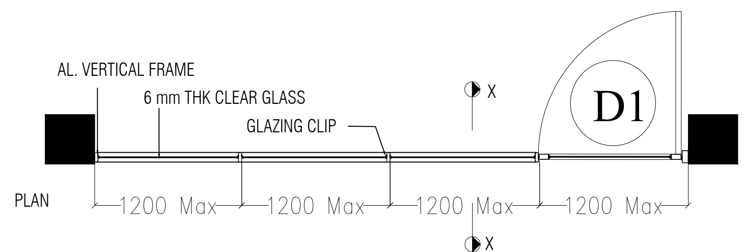
TYPICAL DETAIL FOR INTERIOR ALUMINUM-GLAZING PARTITION
