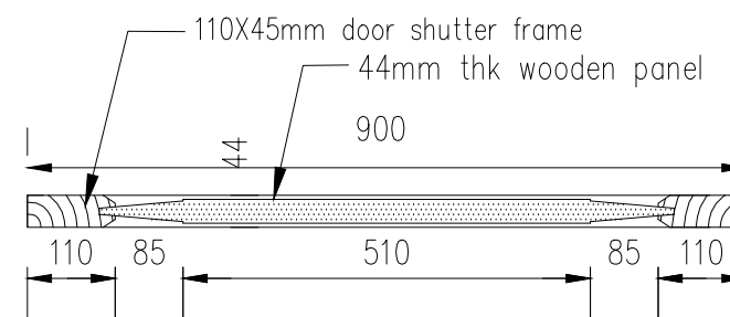
SECTION Y-Y
