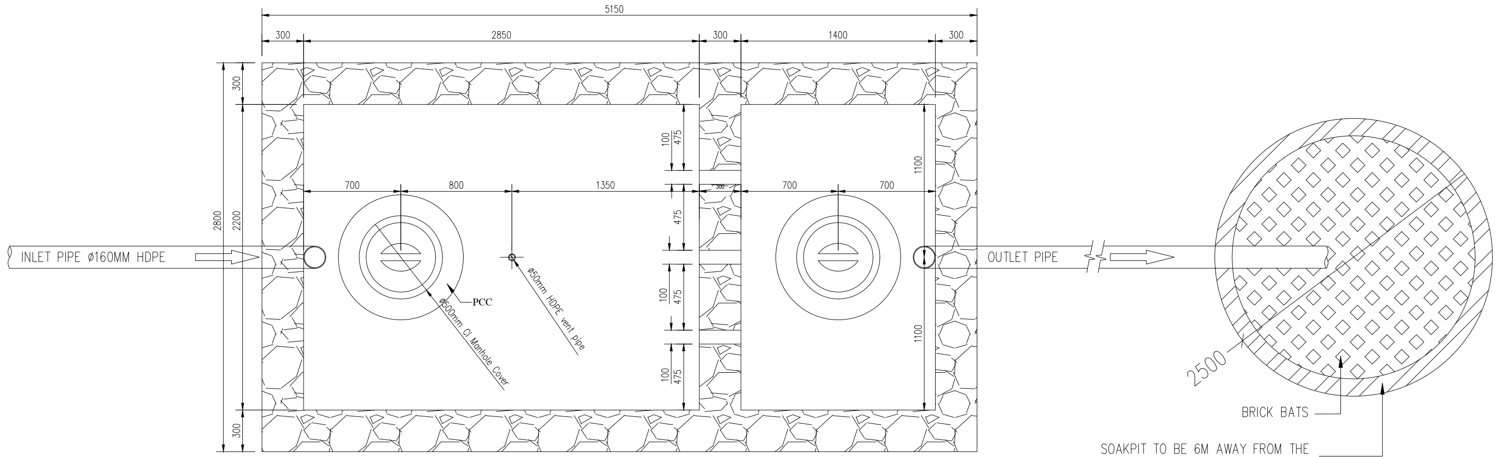
SOAK PIT PLAN
