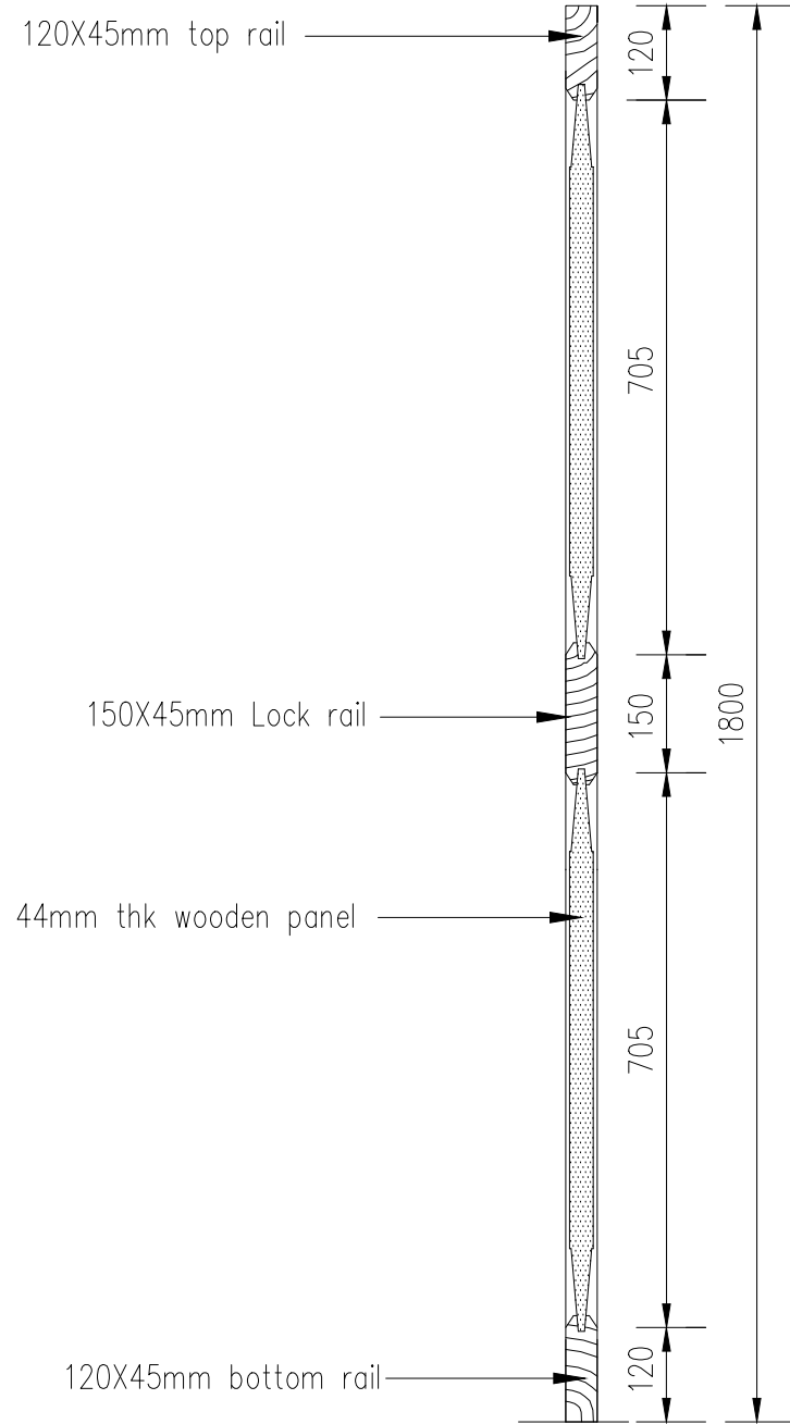
SECTION X-X
