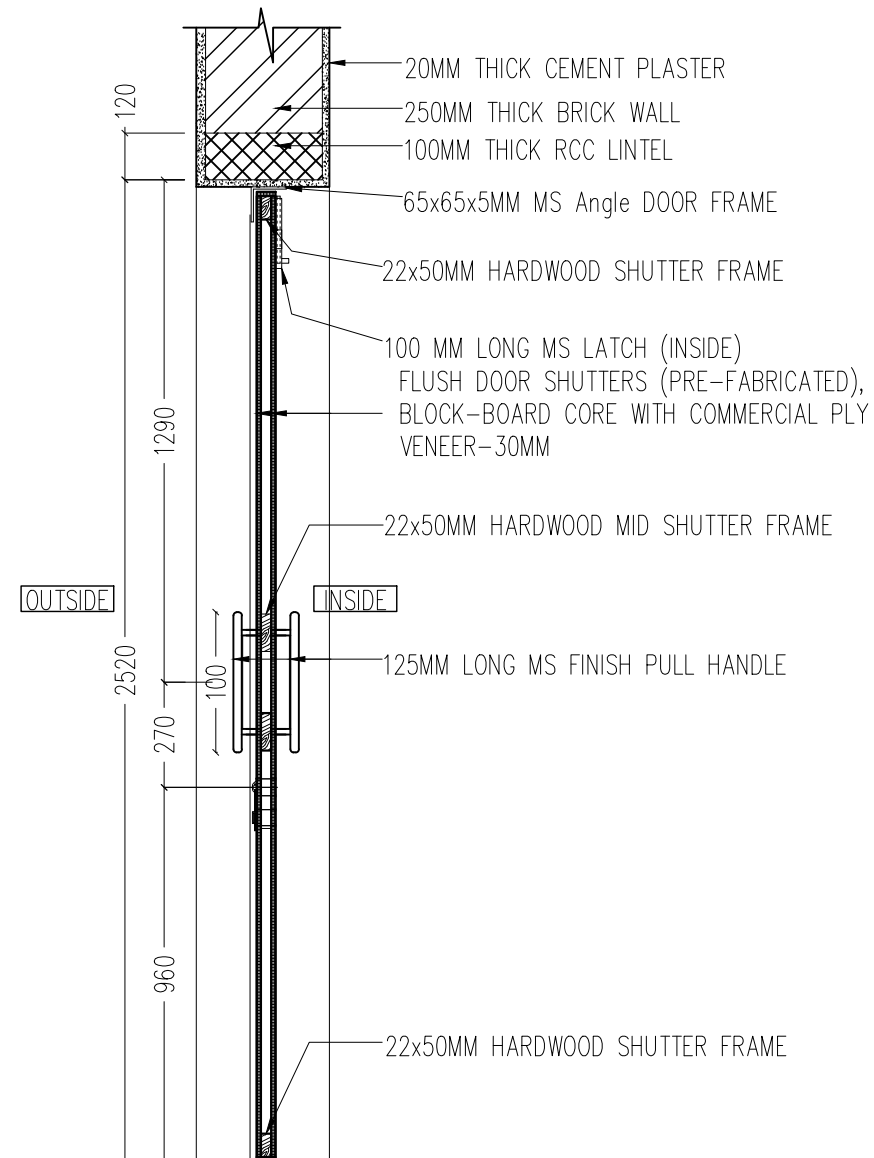
SECTION B-B
