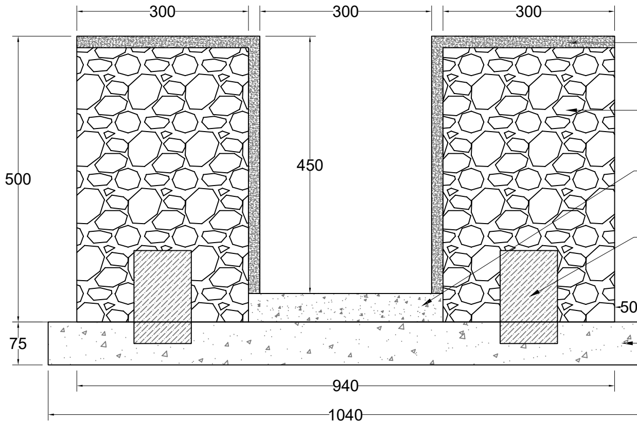
SECTIONAL VIEW OF OPEN SURFACE DRAIN
