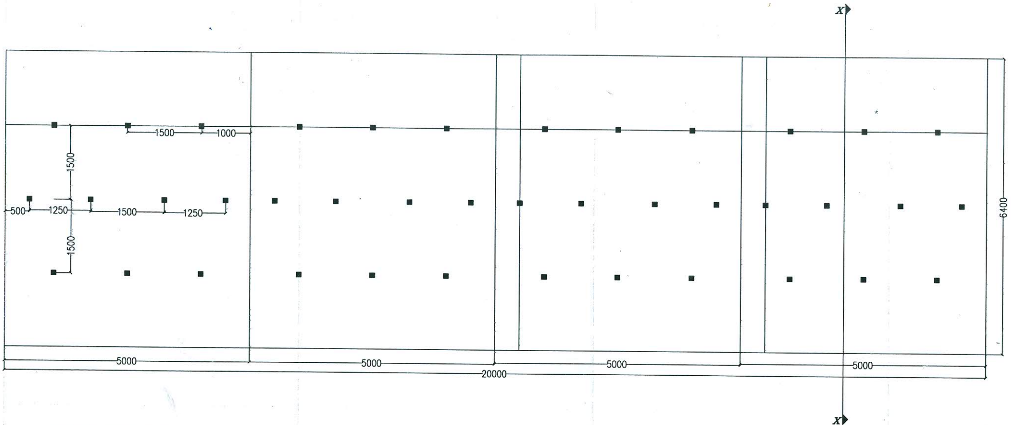
WEEP HOLE LAYOUT FOR THE RRM WALL AT THE APPROACH ROAD OF NGANGLAM SUBSTATION.
