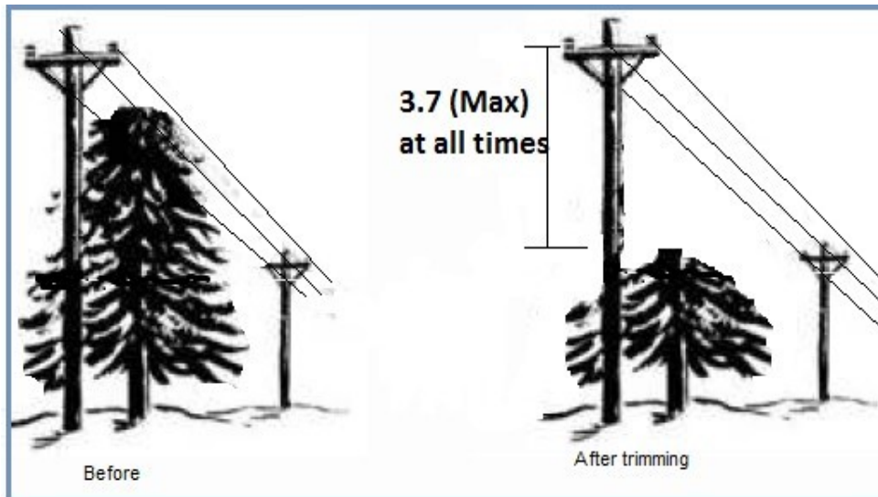
Fig-3: Top trimming (For MV lines)
