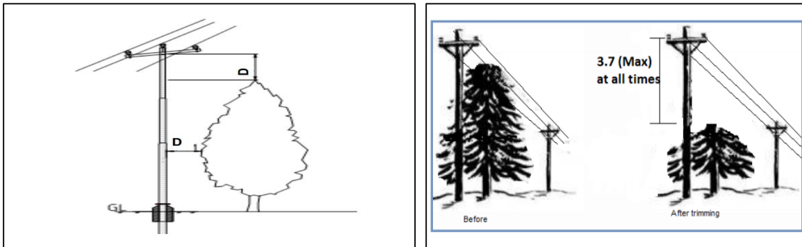
Fig. 2 Top Trimming
