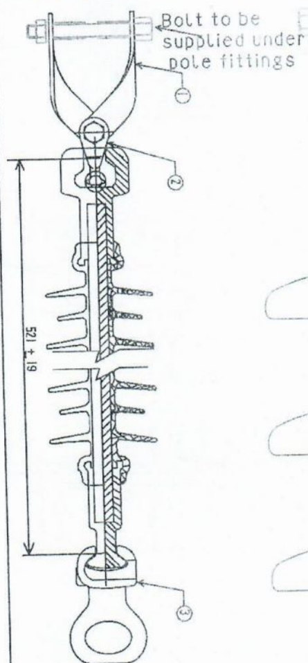
SINGLE TENSION STRING
