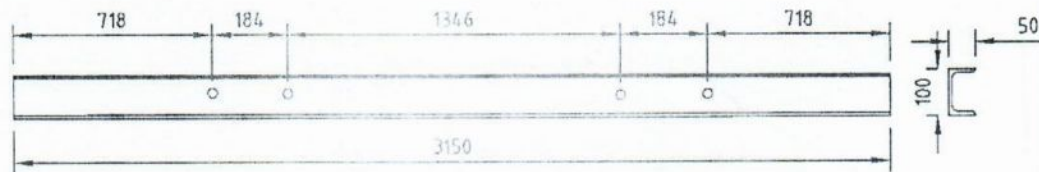
FRONT VIEW OF CROSSARM - CHL
