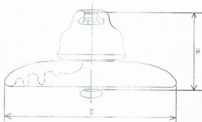
Porcelain Disc Insulator
