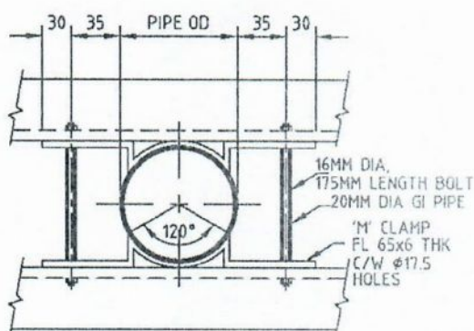
2 'M' CLAMP
