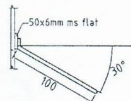
section X-X
