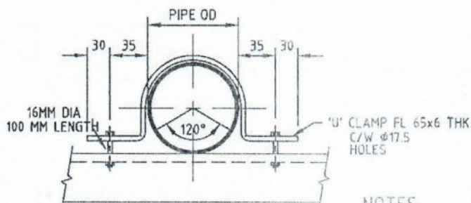
3 FULL CLAMP
