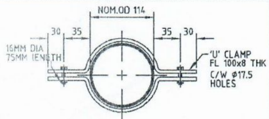
4 STAY CLAMP
