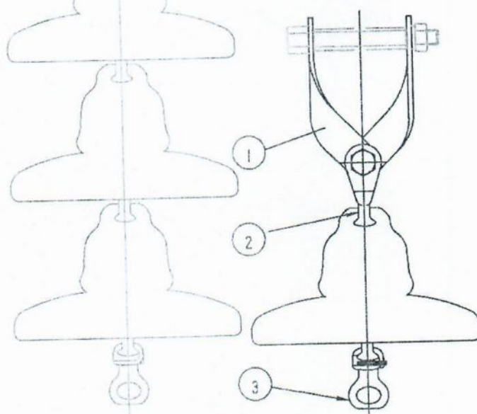
11 kV SINGLE TENSION STRING
