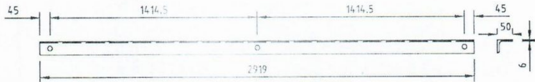
DETAIL OF BRACING - B2
