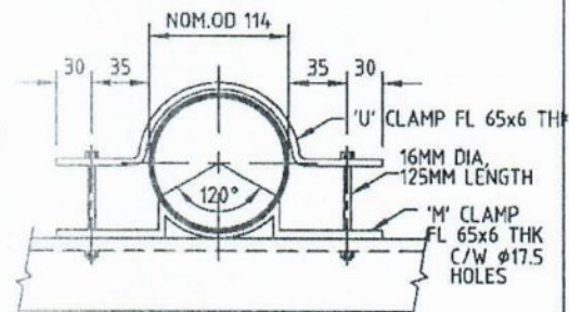
5 CROSS ARM CLAMP (U+M)
