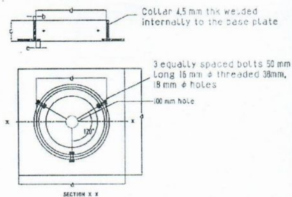
DETAILS OF MS BASE PLATE (Separately packed)
