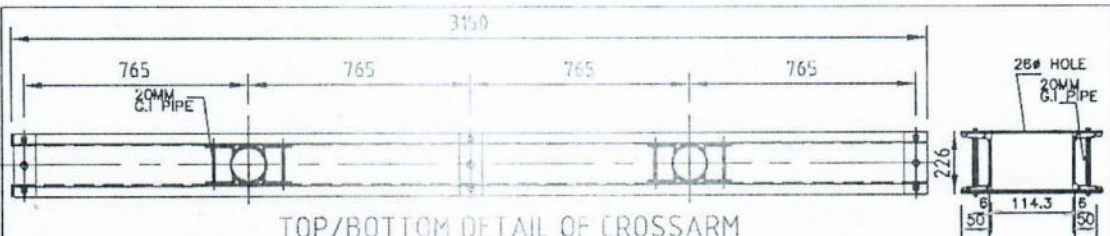
TOP/BOTTOM DETAIL OF CROSSARM
