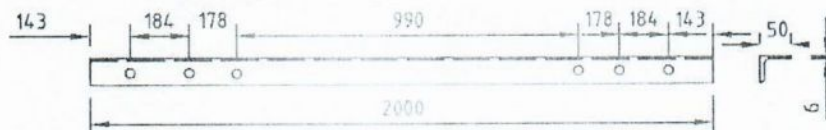
DETAIL OF BRACING - B1
