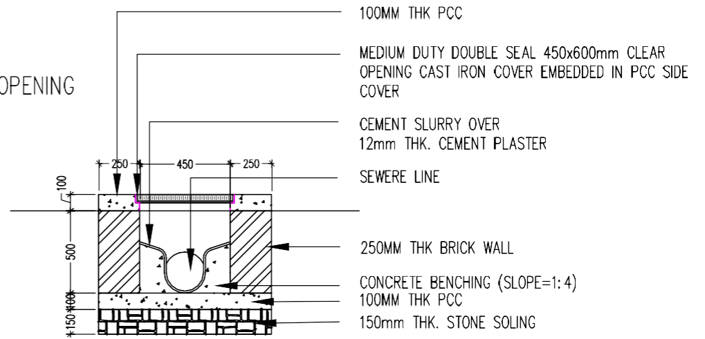
SECTION-MANHOLE CHAMBER
