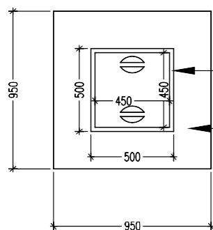
PLAN-MANHOLE CHAMBER
