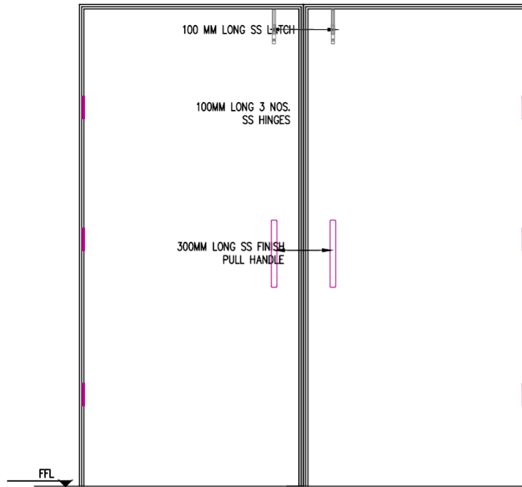
ELEVATION INSIDE
