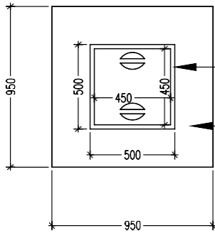
PLAN-MANHOLE CHAMBER
