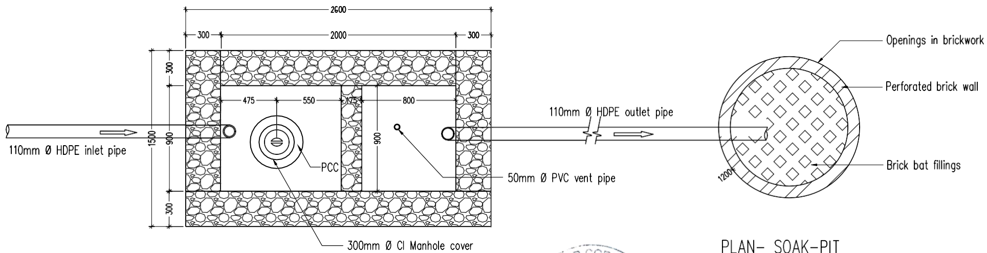
PLAN- SEPTIC TANK FOR 15 USERS
