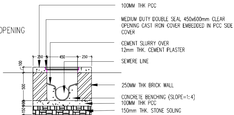
SECTION-MANHOLE CHAMBER
