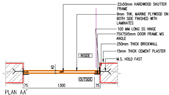
PLAN AA'
