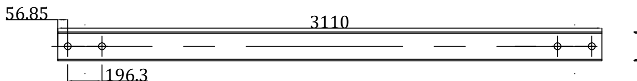
GI SWITCH SUPPORTS FOR ABS, 2NOS. ISMC 100x50-PLAN
