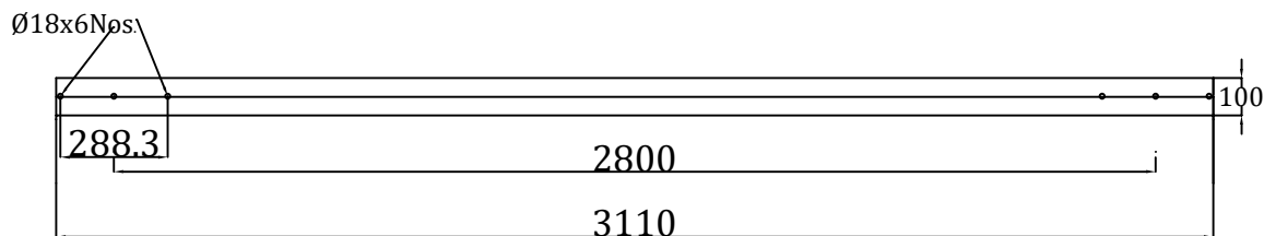
CROSSARM CHANNEL (ISMC 100x50) -ELEVATION
