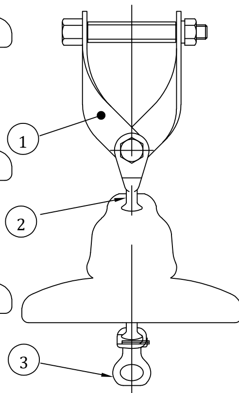
11kV SINGLE TENSION STRING
