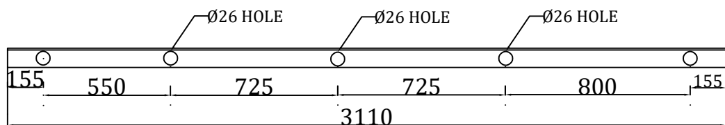
PIN INSULATOR SUPPORTS, 1 NO. ISM 100x50
