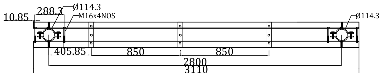
CROSSARM ASSEMBLY
