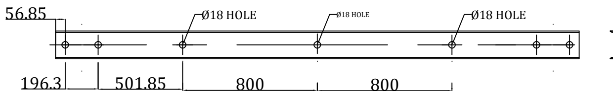
GI SWITCH SUPPORTS FOR ABS, 2NOS. ISMC 100x50
