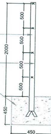
TYPICAL SECTION (SCALE-1:50)
