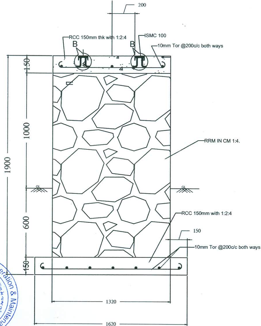
TYPICAL SECTION
