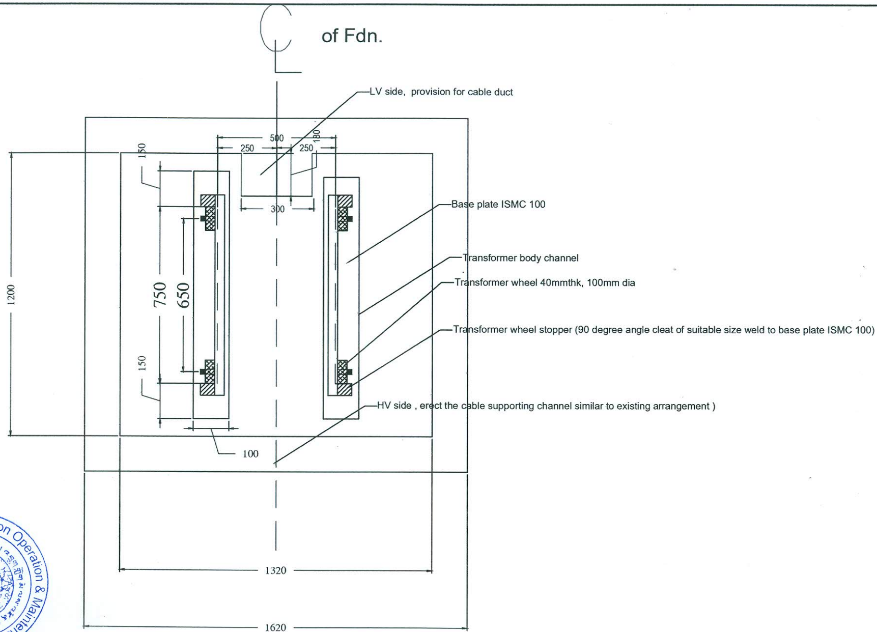
FOUNDATION PLAN
