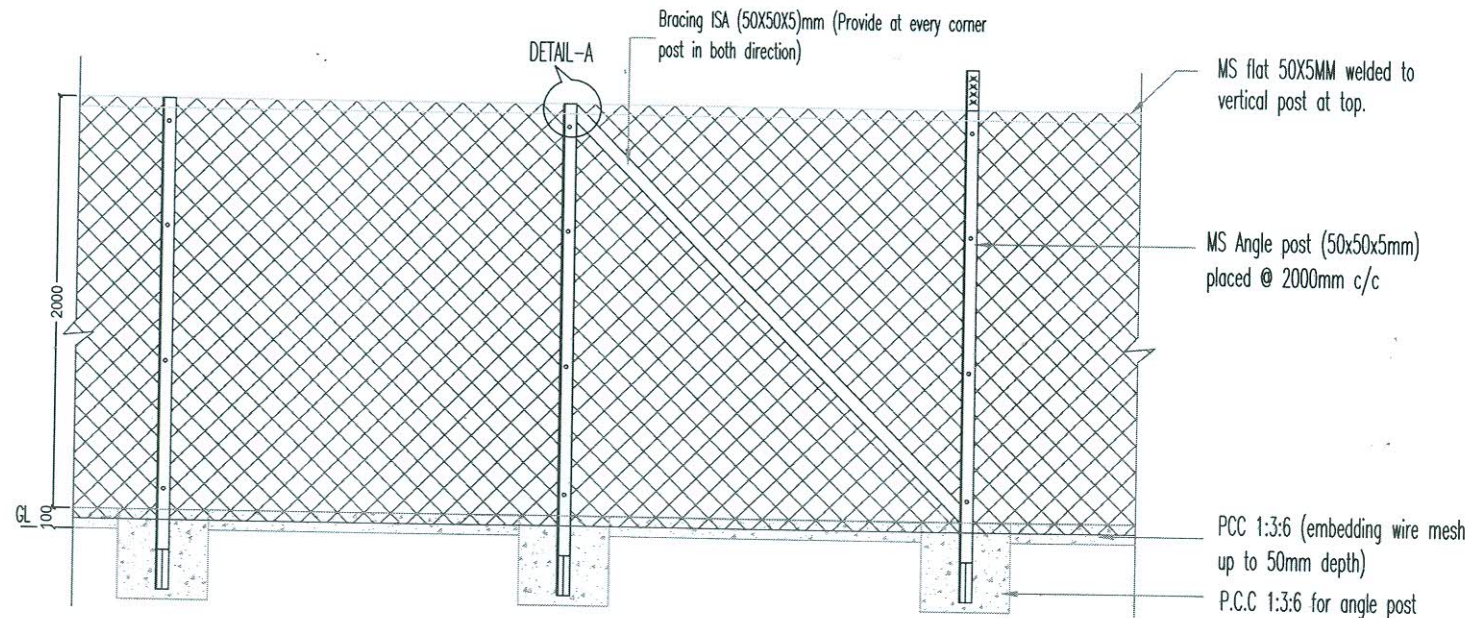
TYPICAL EXTERNAL ELEVATION
