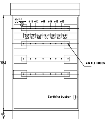
FRONT ELEVATION WITHOUT DOOR
