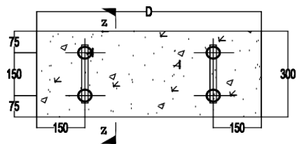
RCC cover slab plan
