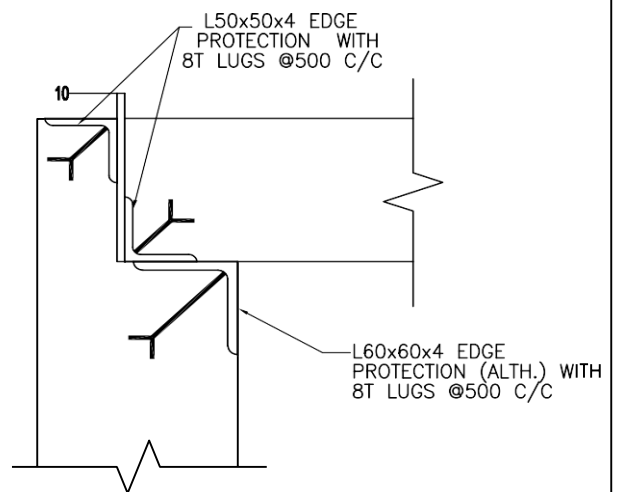
DETAIL Y-Y TYPICAL DETAIL OF CABLE TRENCH EDGE PROTECTION
