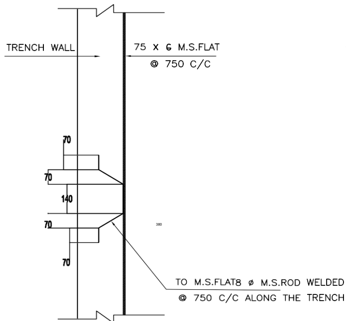
DETAIL X-X : ANCHORING 75x6 M.S. FLAT
