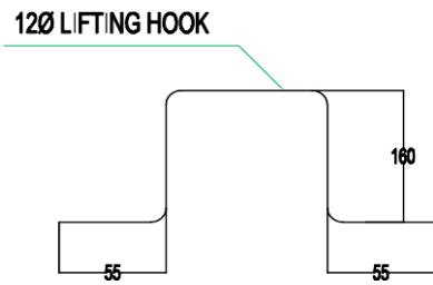
DET. OF LIFTING HOOK
