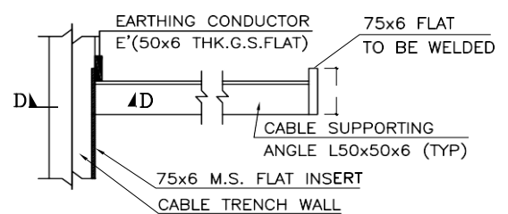
TYP. CABLE SUPPORT EARTH CONDUCTOR E' RUNS ON TOP TIER ONLY
