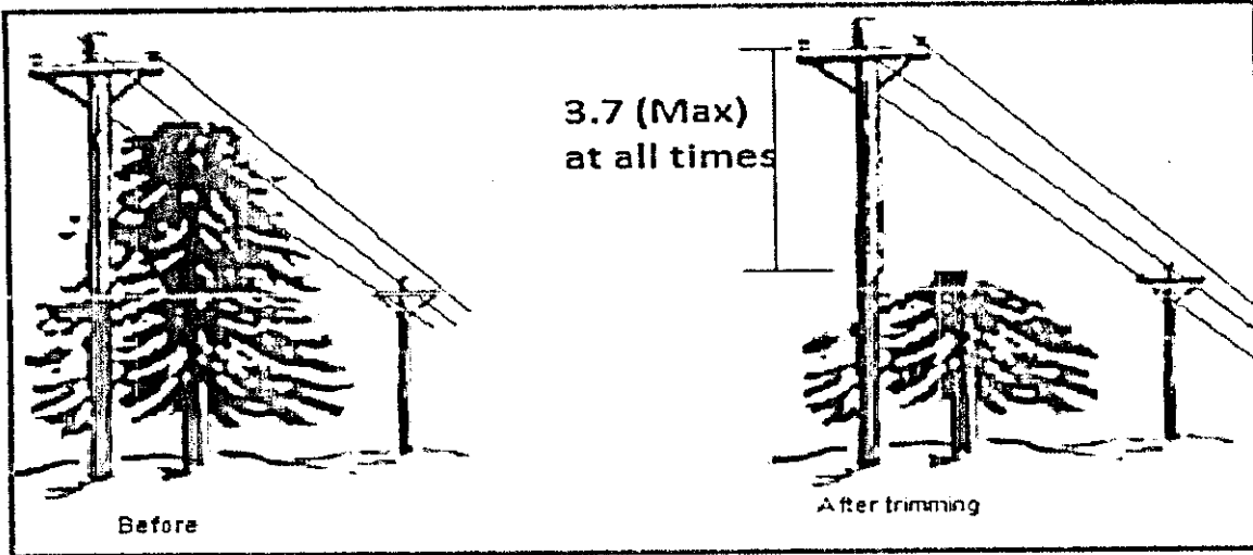
Fig-1: Top Trimming for MV Lines
