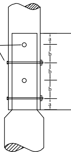
BOLTED JOINT J2 DETAILS
