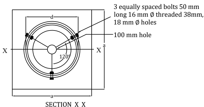
DETAILS OF MS BASE PLATE (Seperately packed)
