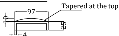
POLE CAP DETAILS (WELDED TO THE POLE)
