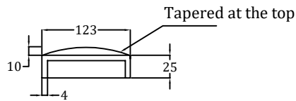
POLE CAP DETAILS(Welded to the pole)
