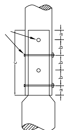
BOLTED JOINT J2 DETAILS
