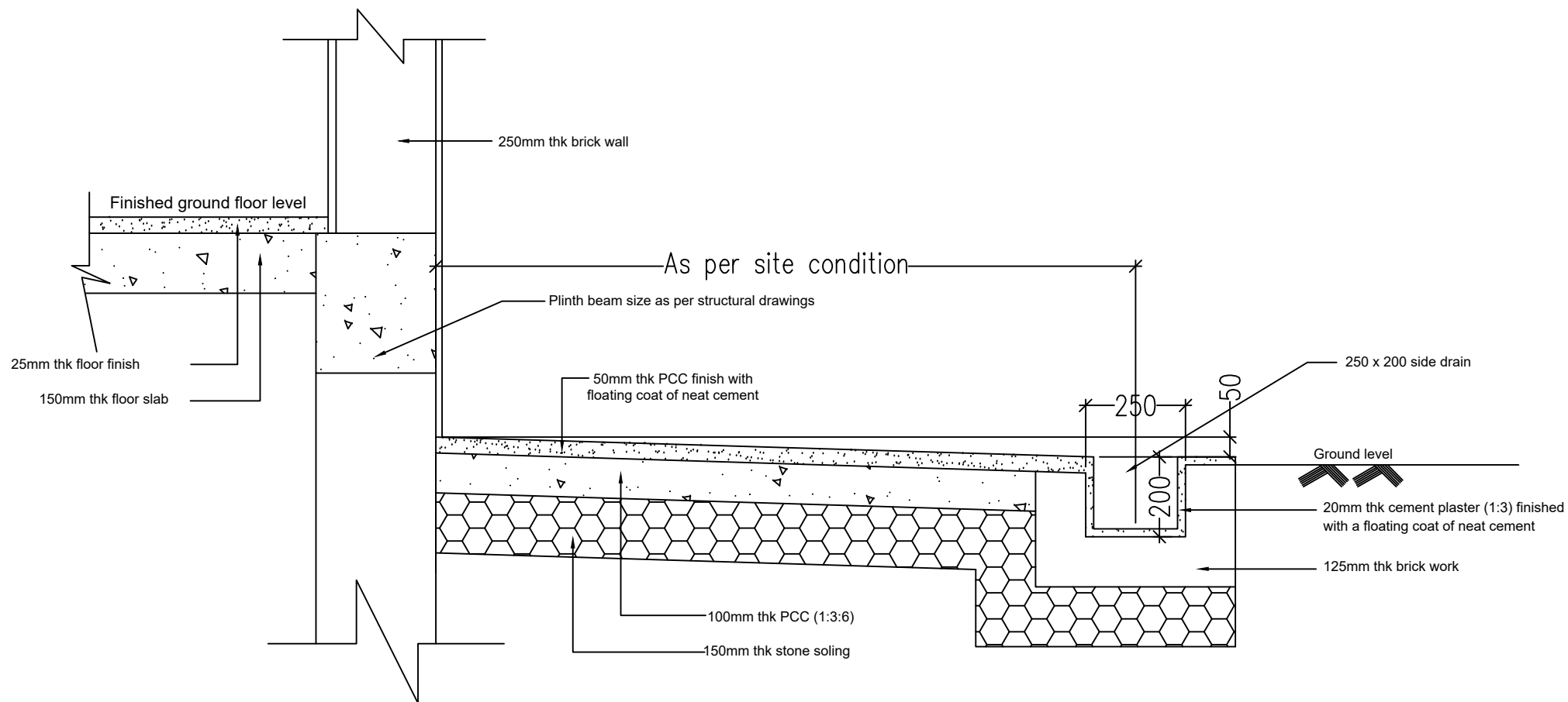
TYPICAL DETAIL OF PLINTH PROTECTION
