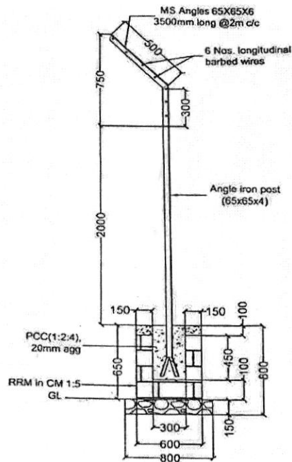
SECTION 1-1
