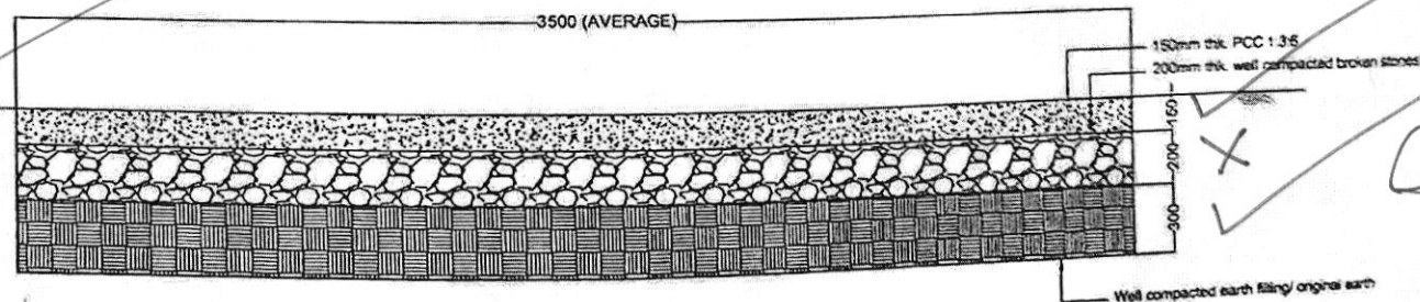
TYPICAL CROSS SECTION OF PCC ROAD
