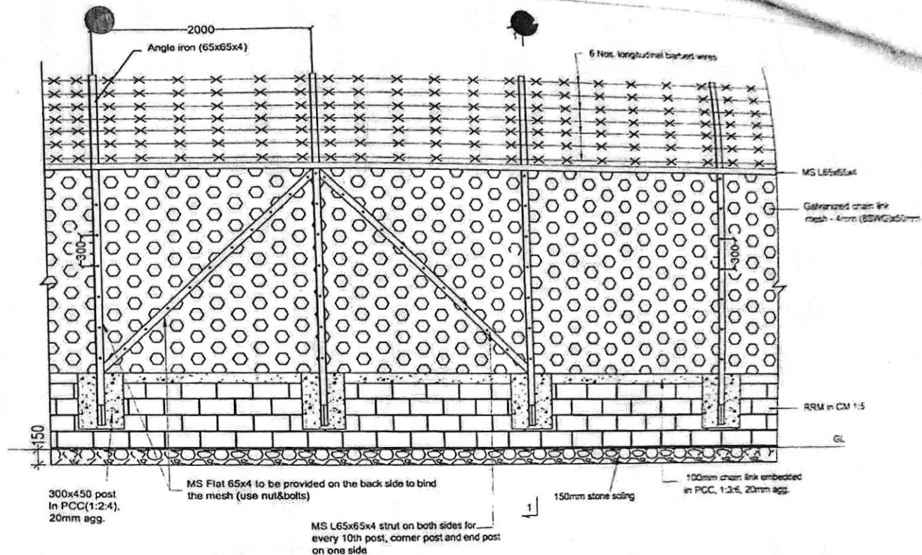
CHAIN LINK FENCING
